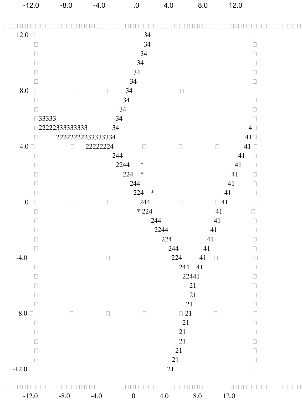
Figure 5. The distribution of the four clusters at the five air quality monitoring work stations
