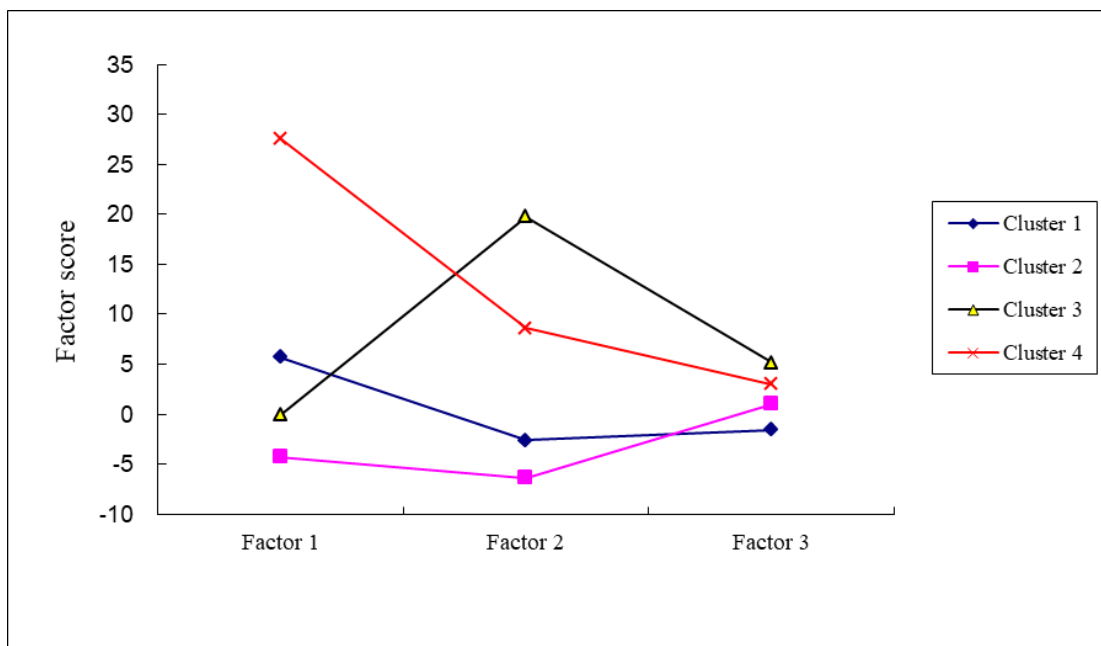
Figure 4. Relationships among clusters and factors
