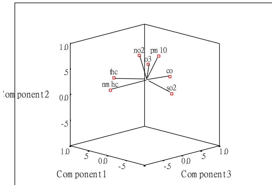
Figure 3. 3D distribution of main factors
